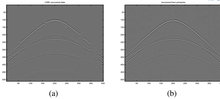
Figure 2: Comparison between CSRI (a) and CSRI + focusing (b) for data with 80% of the traces missing. Notice the significant uplift from compounding the inverse curvelet transform with the focusing 'primary' operator.
