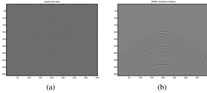
Figure 1: SRME multiple prediction (b) from incomplete data (a) with 80% of the traces missing. Notice the artifacts due to the missing data leading to a deterioration of the multiple prediction.
