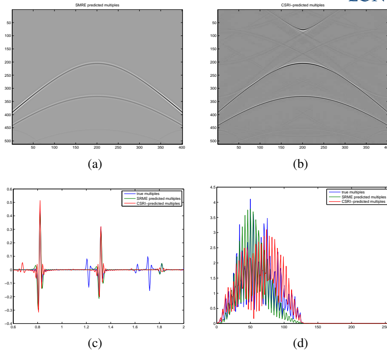
Figure 3: Comparison between convolution-based multiple prediction (a) and sparsity-based multiple prediction (b). Aside from the acausal artifact, the sparsity-promoting multiple prediction according to Eq.5 improves the frequency content and makes it closer to the spectrum of the true multiples. Trace-wise comparisons in (c-d) between the true (including internal) multiples (blue), the multiples predicted with conventional (green) and sparsity promoted predicted multiples (red) confirm this observation. The difference in the spectrum are partially due to the fact that we only predicted the surface-related multiples.
